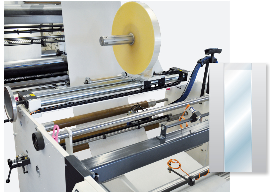
Window unit
